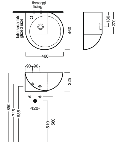
lavabo 46 destro washbasin 92 right
