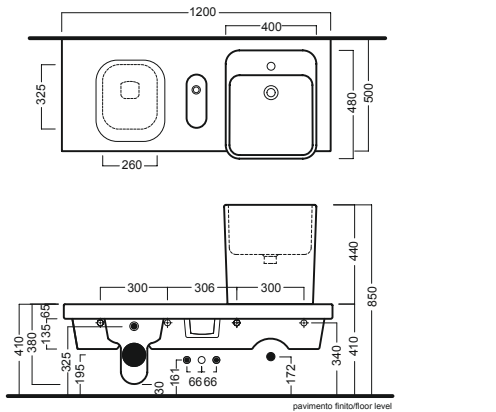
G-FULL 120 vaso a sinistra + lavabo pilozzo G-FULL 140 wc left + sink
