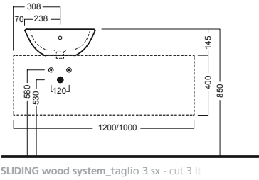
SLIDING wood system_taglio 3 sx - cut 3 lt
