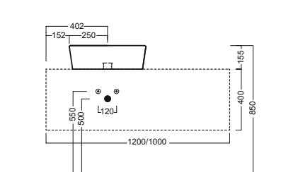
SLIDING wood system_taglio 2 sx - cut 2 lh
