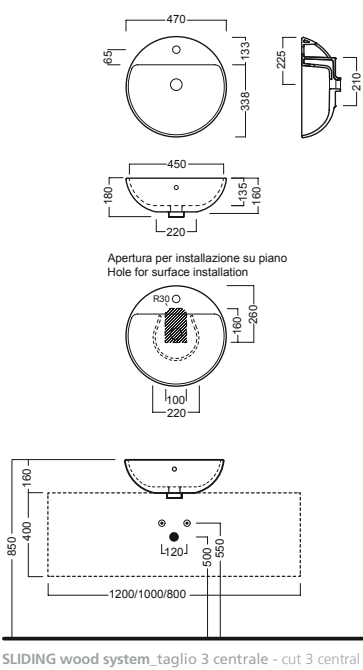
SLIDING wood system_taglio 3 centrale - cut 3 central
