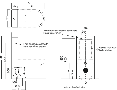
cassetta attacco posteriore back inlet cistern
