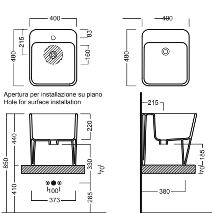
lavabo pilozzo in appoggio surface-mounted sink
