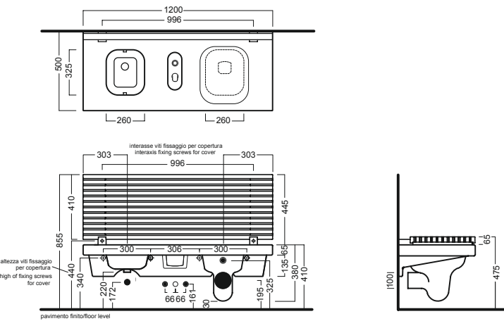
G-FULL 120 vaso a destra G-FULL 120 wc right
