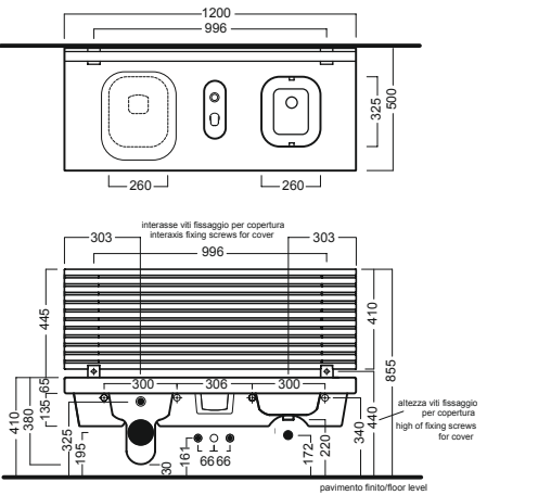
G-FULL 120 vaso a sinistra G-FULL 120 wc left
