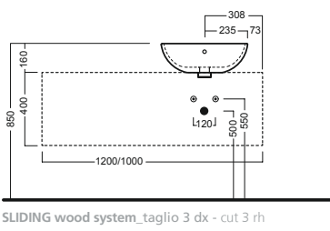
SLIDING wood system_taglio 3 dx - cut 3 rh
