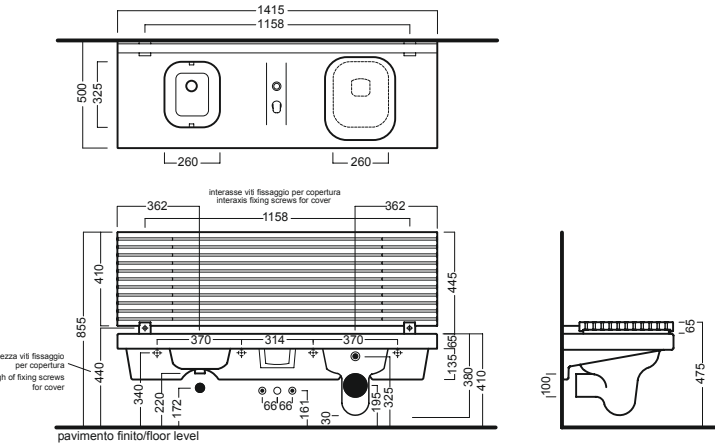
G-FULL 140 vaso a destra G-FULL 140 wc right
