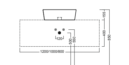
SLIDING wood system_taglio 2 centrale - cut 2 central
