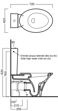
vaso monoblocco con cassetta coupled wc with cistern
