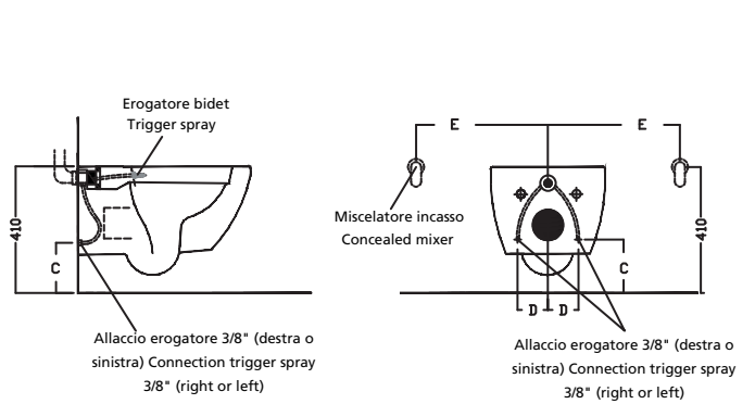
Vaso Sospeso-Wall-hung WC-Hang Wc
