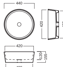
lavabo 07:00 washbasin 07:00
