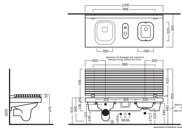
G-FULL 120 vaso a sinistra G-FULL 120 wc left
