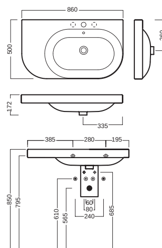
lavabo 86 destro washbasin 86 right
