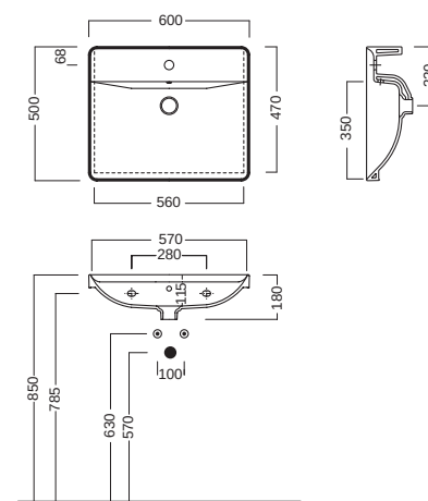
lavabo 60 washbasin 60
