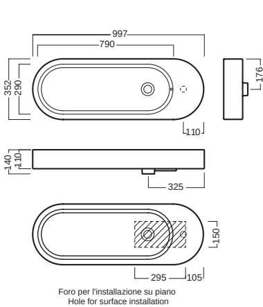
lavabo 100x35 washbasin 100x35
