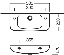
lavamani DINO DINO handrinse basins
