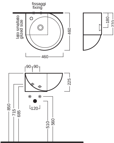
lavabo 46 destro washbasin 92 right
