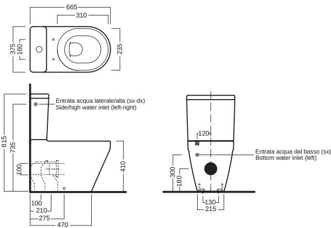
vaso monoblocco con cassetta coupled wc with cistern
