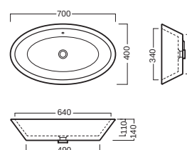
lavabo 22:00 washbasin 22:00
