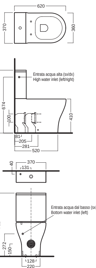
vaso monoblocco con cassetta coupled wc with cistern
