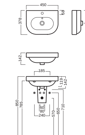
lavabo 45 washbasin 45
