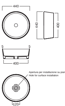
lavabo 07:00s washbasin 07:00s
