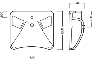
lavabo ergonomico ergonomic washbasin
