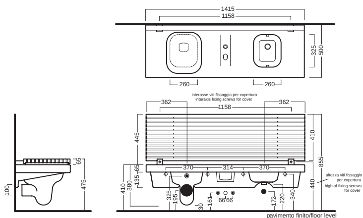
G-FULL 140 vaso a sinistra G-FULL 140 wc left
