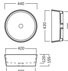
lavabo 07:15 washbasin 07:15
