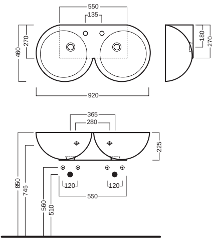
lavabo 92 washbasin 92
