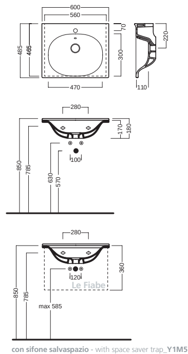
lavabo 60 washbasin 60
