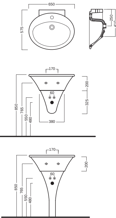
lavabo 65 washbasin 65
