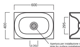
lavabo 60 washbasin 60
