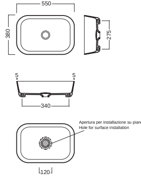
lavabo 18:00s washbasin 18:00
