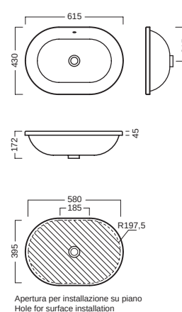
lavabo 62 incasso 62 countertop washbasin
