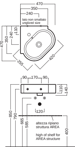
lavabo 47x47 destro washbasin 80x35 right
