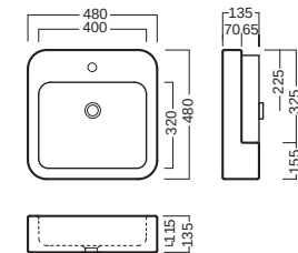
lavabo 09:30 washbasin 09:30
