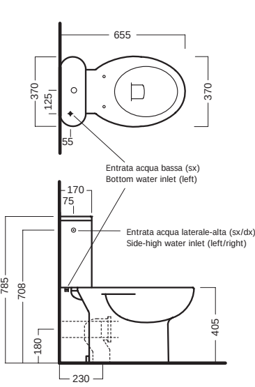
vaso monoblocco con cassetta coupled wc with cistern
