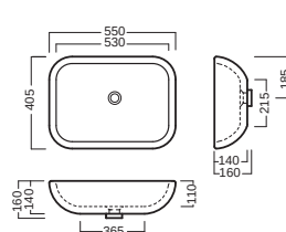
lavabo 17:00 washbasin 17:00
