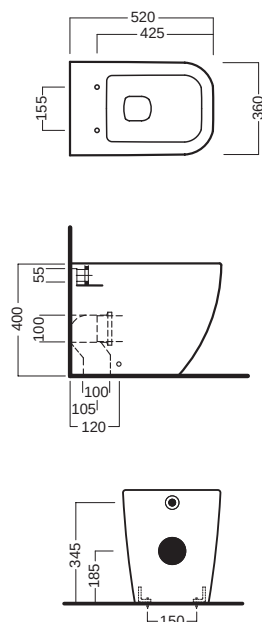
vaso filo muro back to wall wc
