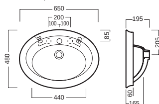
lavabo 65 ad incasso countertop washbasin 65
