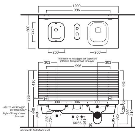
G-FULL 120 vaso a destra G-FULL 120 wc right
