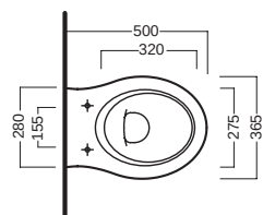
vaso filo muro_50 back to wall wc_50
