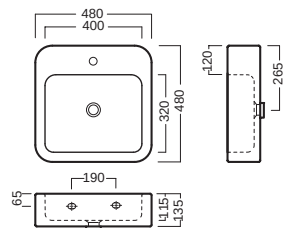
lavabo 09:00 washbasin 09:00
