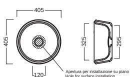
lavabo 40 washbasin 40
