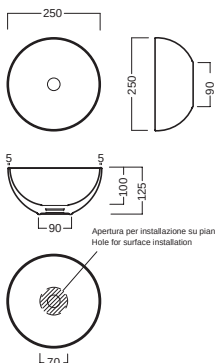
lavabo 05:00s washbasin 05:00s
