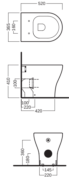
vaso filo muro back to wall wc
