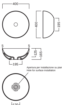
lavabo 06:00s washbasin 06:00s
