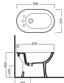
bidet triforo three holes bidet
