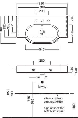
lavabo 81x45 washbasin 81x45
