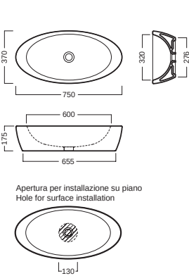
lavabo 75 da appoggio surface-mounted washbasin 75
